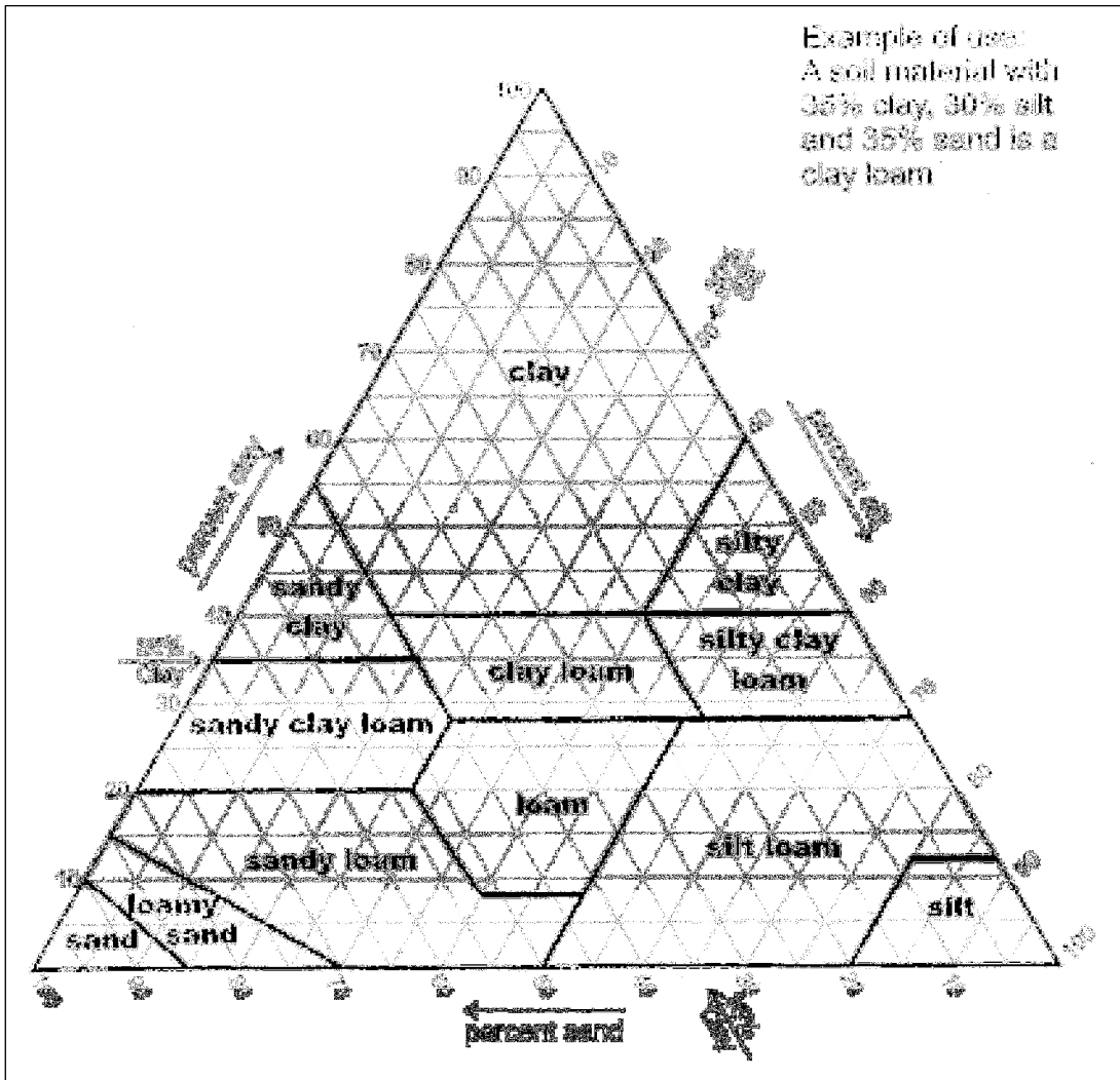
Figure 1. US Department of Agriculture textural classification of soils
